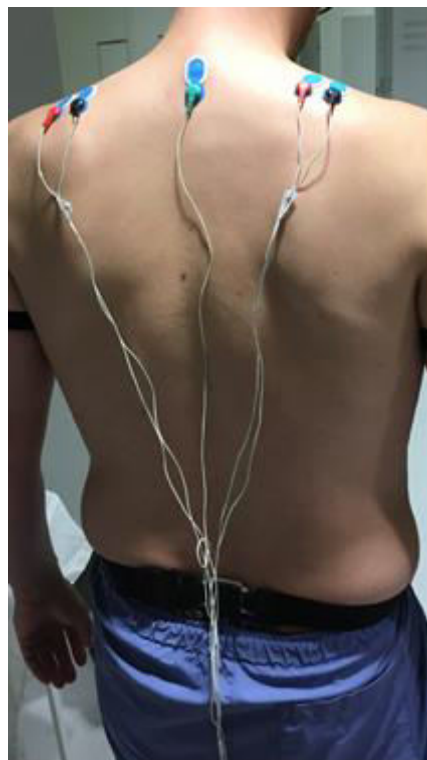
Figure 3. Electromyography surface electrodes on the descending trapezius muscle. Green is the ground.
